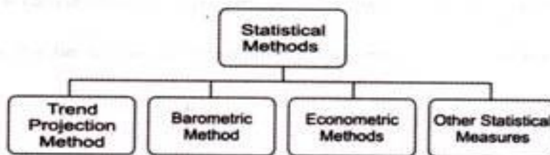
Figure-12: Statistical Methods
